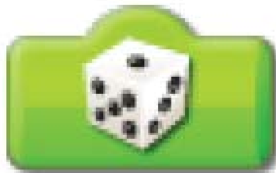
Random Input
